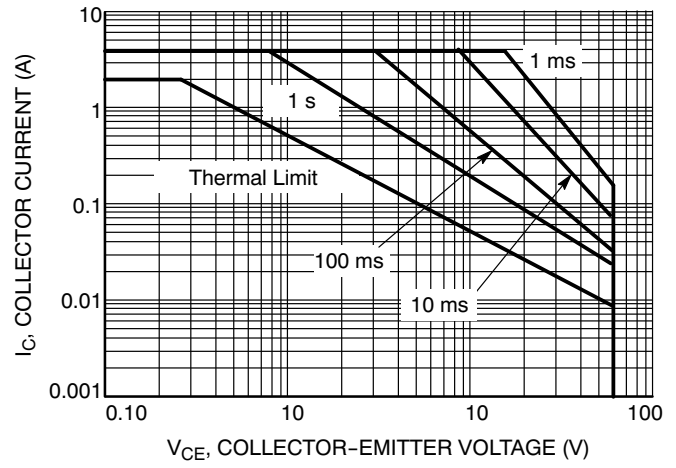
Figure 8. Safe Operating Area Single Pulse Test @ T_{\text{amb}} = 25^\circ\text{C}
